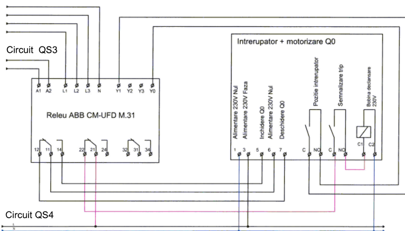
Circuit F01
