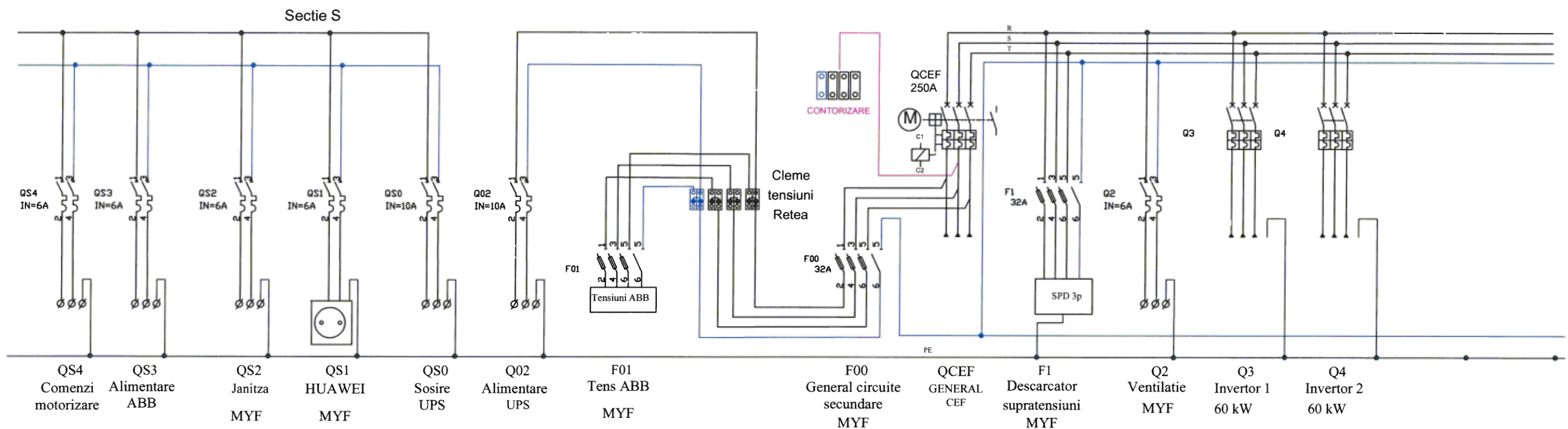
Circuit F01
